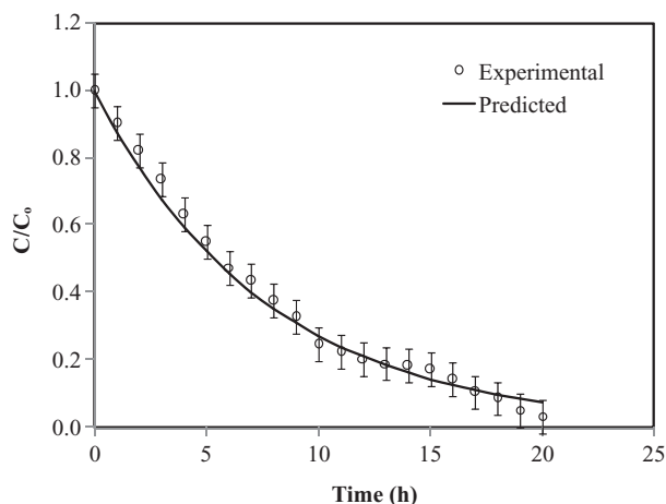
Fig. 5. Comparison of experimental values with predicted values (using Eq. (1)) (PTFE impregnated with coconut oil, RPM 350, Feed pH 4, feed concentration 1,000 mg/L, strip (NaOH) solution concentration 0.2 M.
