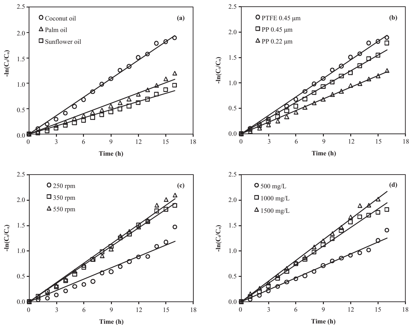
Fig. 3. (a) Effect of different triglycerides (vegetable oils, PTFE, pore size 0.45\ \mu\text{m} , feed pH 4.0, RPM 350, feed concentration 1,000\ \text{mg/L} , strip concentration 0.2\ \text{M} ); (b) type of membranes (support material impregnated with coconut oil, feed pH 4, RPM 350, feed concentration 1,000\ \text{mg/L} , strip concentration 0.2\ \text{M} ), (c) stirring speed (PTFE impregnated with coconut oil, feed pH 4, feed concentration 1,000\ \text{mg/L} , strip concentration 0.2\ \text{M} ) and, (d) initial phenol concentration on the mass transfer coefficient of phenol (PTFE impregnated with coconut oil, RPM 350, Feed pH 4, strip concentration 0.2\ \text{M} )
