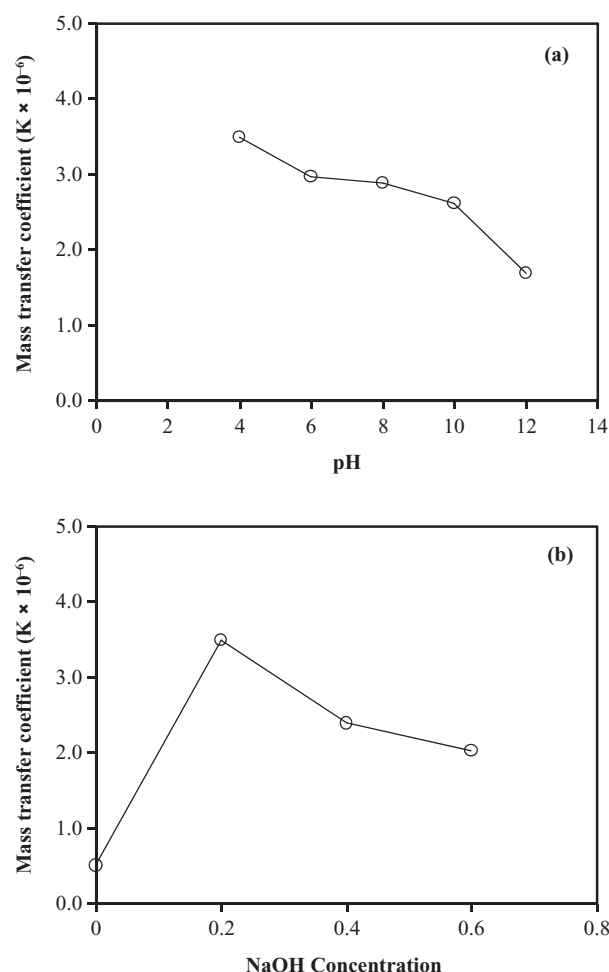
Fig. 4. (a) Effect of pH on the mass transfer coefficient of phenol (PTFE impregnated with coconut oil, RPM 350, feed conc. 1,000 mg/L, strip conc. 0.2 M); (b) effect of strip (NaOH) solution concentration on the mass transfer coefficient of phenol (PTFE impregnated with coconut oil, RPM 350, Feed pH 4, feed concentration. 1,000 mg/L).
