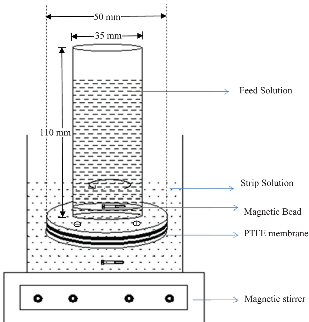
Fig. 2. Schematic design of supported liquid membrane (SLM) model.
