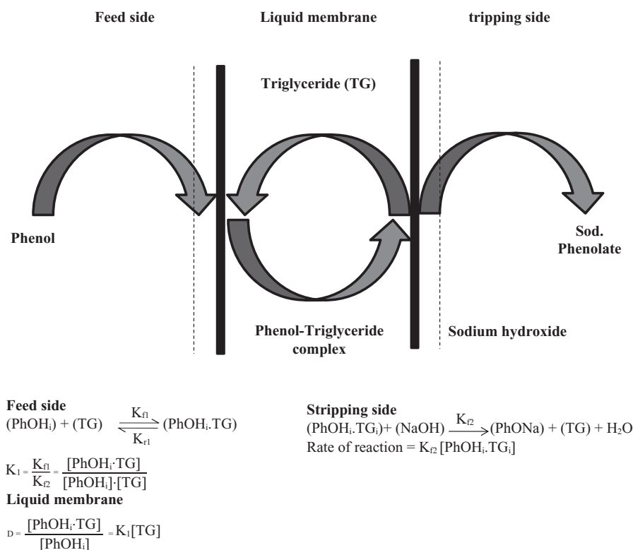
Fig. 1. Mechanism of mass transfer of phenol through supported liquid membrane using vegetable oils. Dotted lines show the boundary layers on feed as well as stripping side. [\text{PhOH}] and [\text{PhOH}_i] are concentrations of phenol in bulk and feed side boundary layer, respectively. [\text{PhOH}_i \cdot \text{TG}] and [\text{PhOH}_i \cdot \text{TG}_i] are concentrations of phenol-triglyceride complex in liquid membrane and stripping side boundary layer, respectively. K_{f1} and K_{r2} are the rate of forward and backward reaction on feed side. K_{r1} is the rate of disappearance of phenol-triglyceride complex on stripping side, respectively. D is the distribution coefficient of phenol in aqueous and triglyceride phase.
